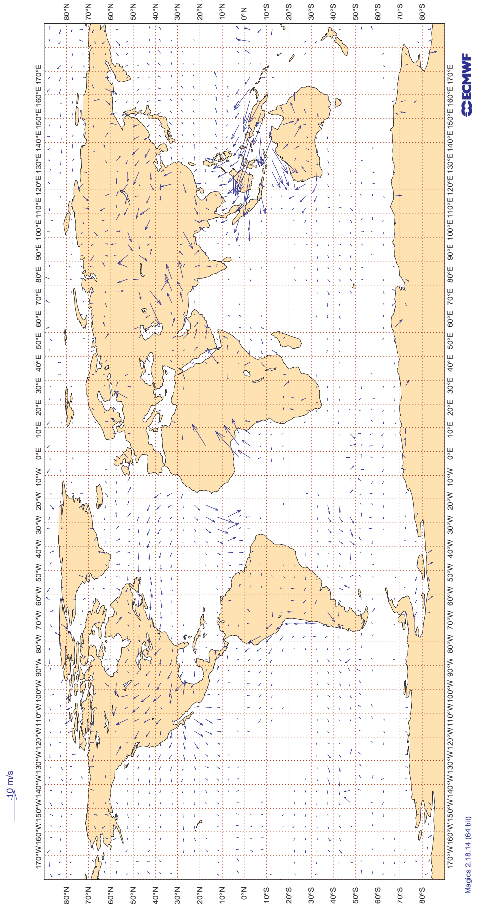
Figure 16 ECMWF Monitoring Statistics: Feb 2014 AMV Winds: 700-1000hPa Wind bias: Observation - FG
