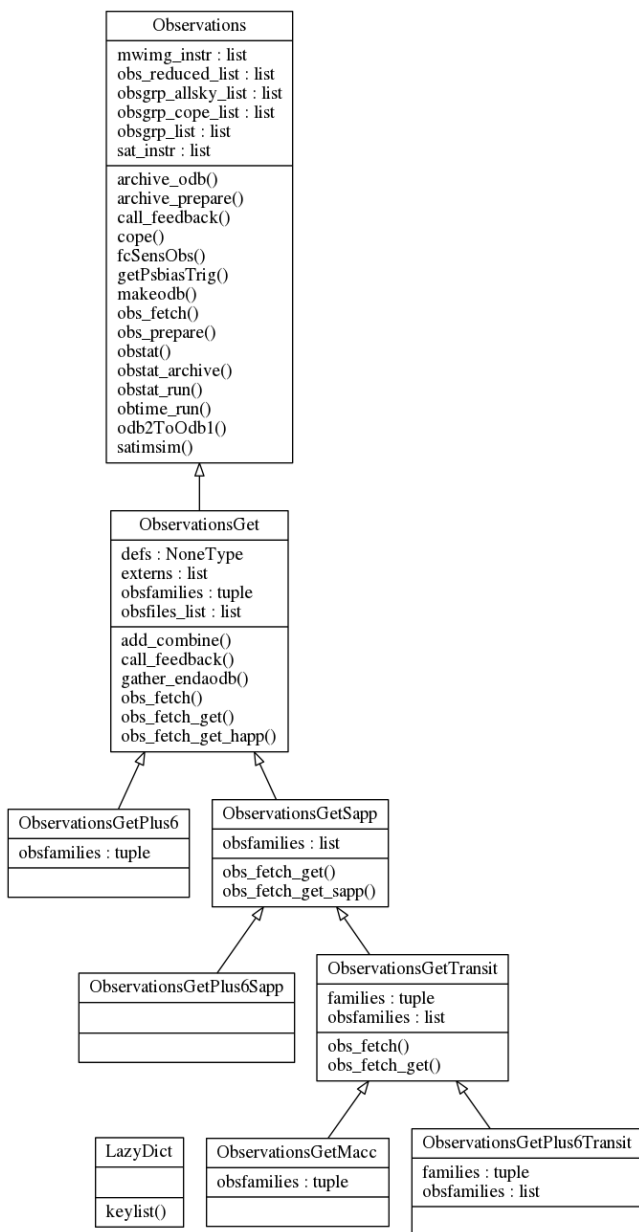
Figure 3.6 Class Diagram for module inc_obs.py .
