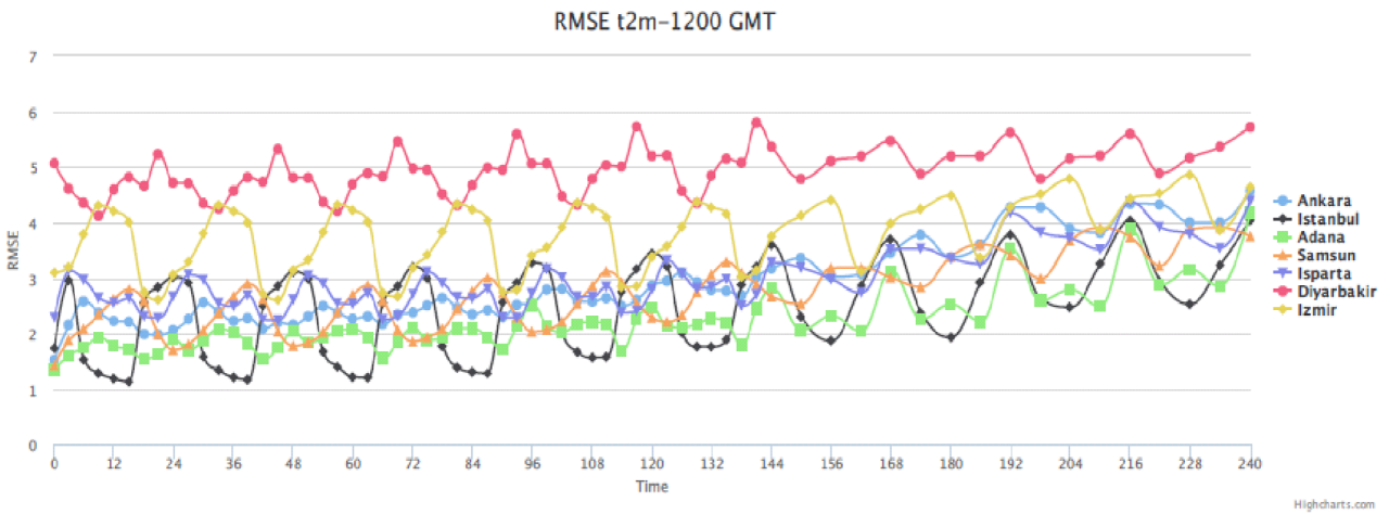
Fig. 11 RMSE of 12 UTC 2m temperature forecasts as a function of forecast range for 7 Turkish radio-sonde stations
