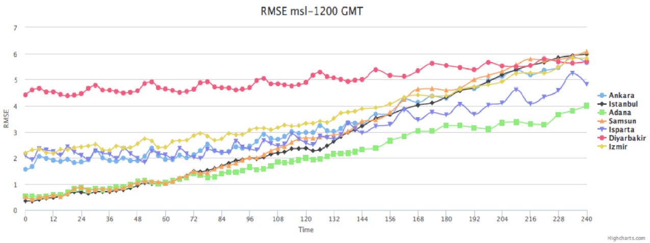
Fig. 9 RMSE of 12 UTC MSLP forecasts as a function of forecast range for 7 Turkish radio-sonde stations
