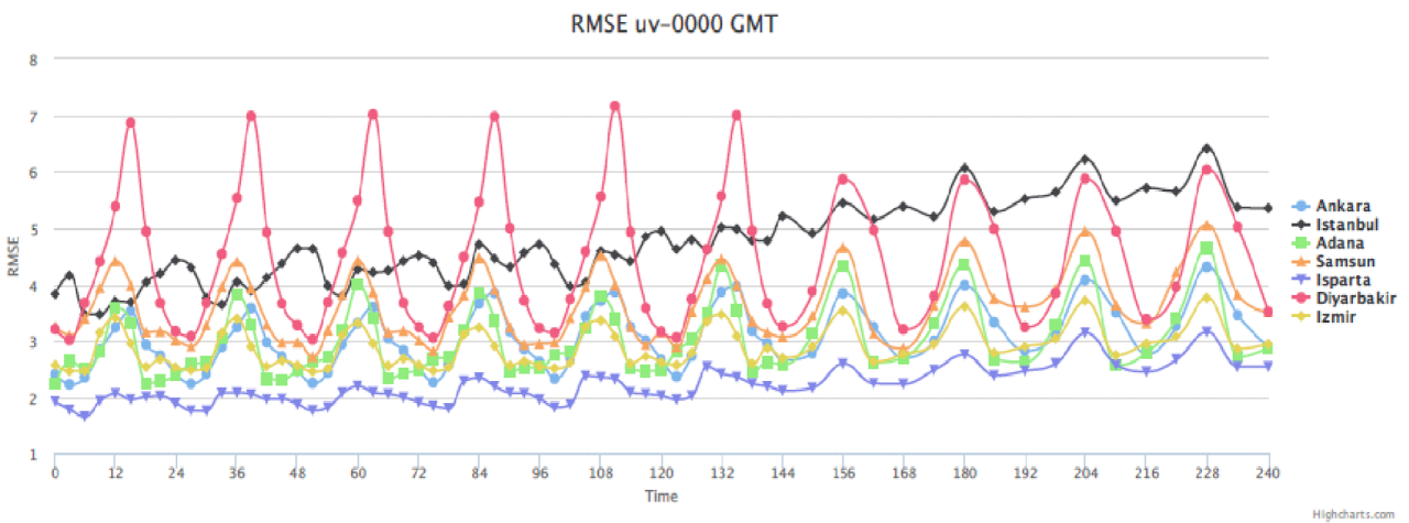
Fig. 12 RMSE of 00 UTC wind speed forecasts as a function of forecast range for 7 Turkish radio-sonde stations
