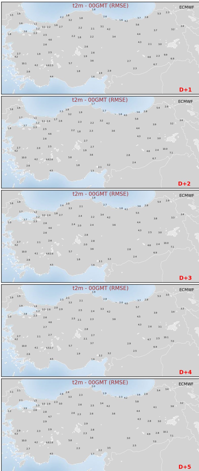
Fig. 4 00 UTC RMSE Values of 2m temperature for D+1 to D+5
