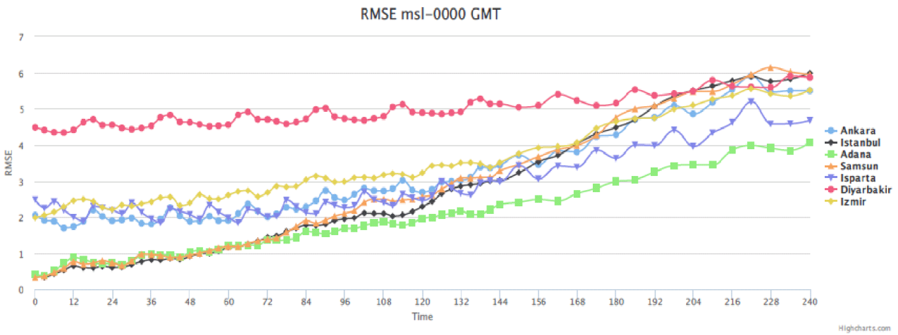
Fig. 8 RMSE of 00 UTC MSLP forecasts as a function of forecast range for 7 Turkish radio-sonde stations
