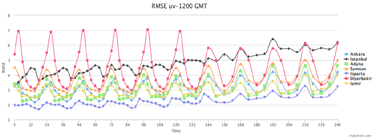
Fig. 13 RMSE of 12 UTC wind speed forecasts as a function of forecast range for 7 Turkish radio-sonde stations
