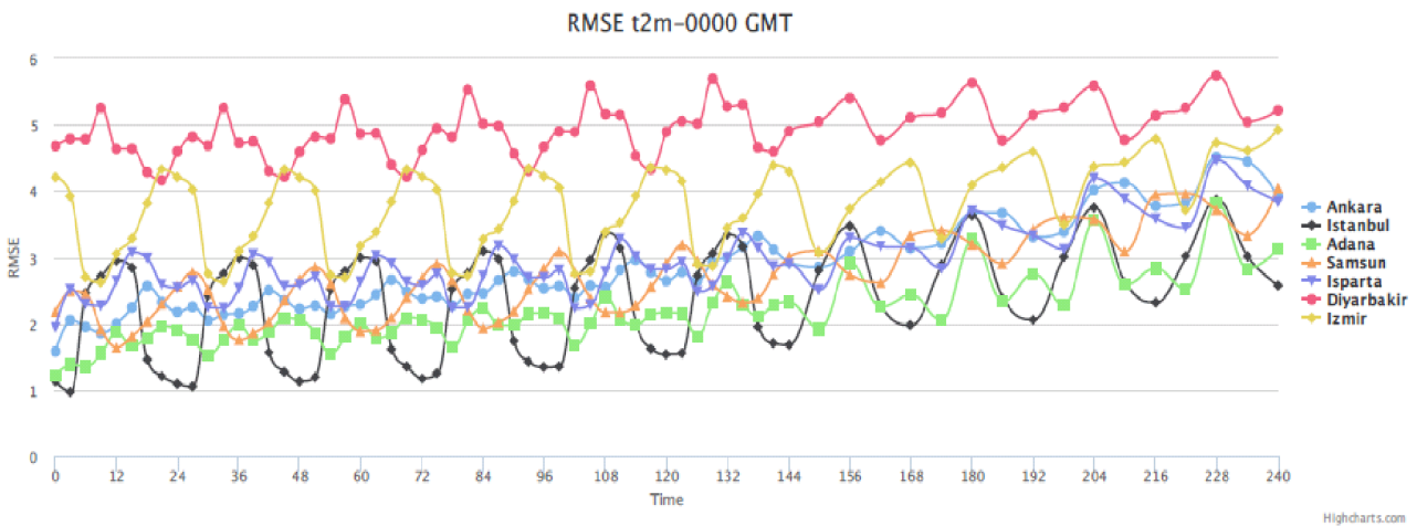
Fig. 10 RMSE of 00 UTC 2m temperature forecasts as a function of forecast range for 7 Turkish radio-sonde stations
