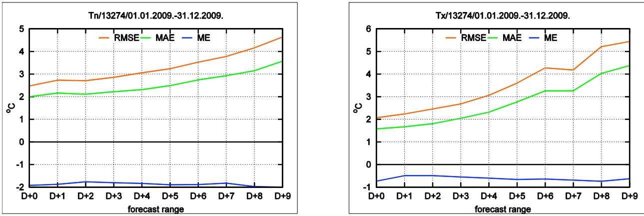
Fig.1-2 ME, MAE and RMSE of ECMWF 2m minimum and maximum temperature forecast (D+0 to D+9) as a function of forecast range (Beograd - Karađorđev park).
