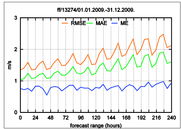
Fig.5-6 ME, MAE and RMSE of ECMWF 2m temperature and 10m wind speed forecast as a function of forecast range (Beograd - Karađorđev park).
