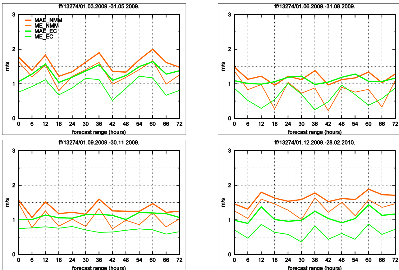
Fig.13-20 ME and MAE of 2m temperature and 10m wind speed forecast as a function of forecast range. Comparison of ECMWF to WRF-NMM forecasts for seasons MAM09 to DJF10 (Beograd - Karađorđev park).
