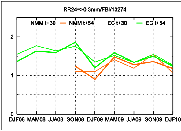
Fig.11-12 FBI and KSS of ECMWF 24h precipitation forecast (t+30h and t+54h) for seasons DJF08 to DJF10. Threshold is 0.3mm/24h. Comparison to WRF-NMM forecast from SON08 (Beograd - Karadordev park).
