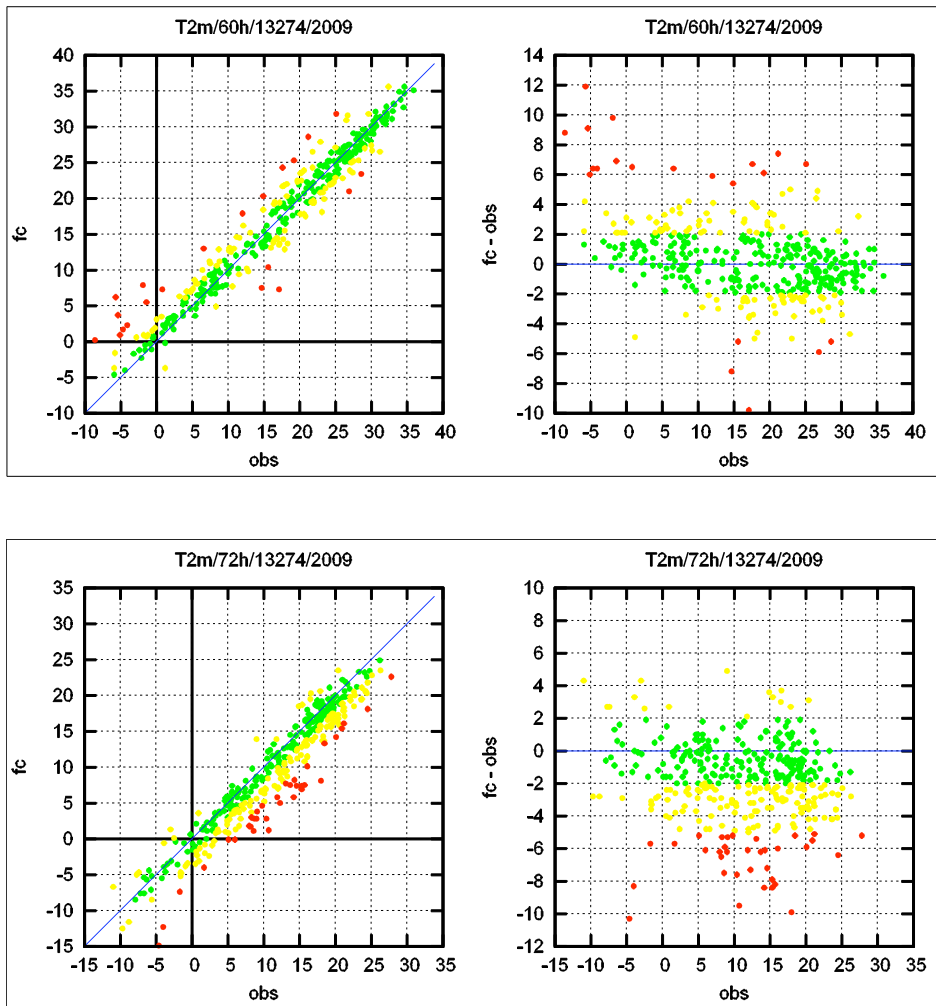
Fig.3-4 Scatterplots and forecast errors vs. observations of one year ECMWF t+60h (midday) and t+72h (midnight) 2m temperature forecast for Beograd - Karađorđev park (13274).
