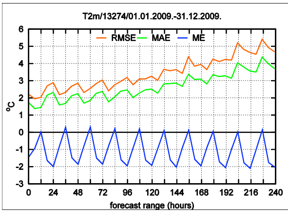
Fig.5-6 ME, MAE and RMSE of ECMWF 2m temperature and 10m wind speed forecast as a function of forecast range (Beograd - Karađorđev park).
