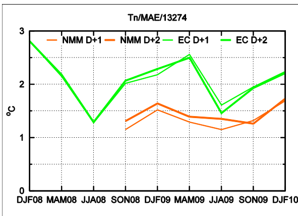
Fig.7-10 ME and MAE of ECMWF 2m minimum (t+30 for D+1 and t+54 for D+2) and maximum (t+42 for D+1 and t+66 for D+2) temperature forecast for seasons DJF08 to DJF10. Comparison to WRF-NMM forecast for three last seasons (Beograd - Karađorđev park).
