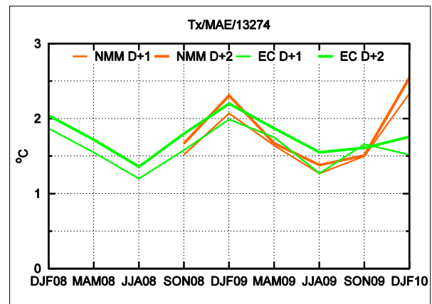
Fig.7-10 ME and MAE of ECMWF 2m minimum (t+30 for D+1 and t+54 for D+2) and maximum (t+42 for D+1 and t+66 for D+2) temperature forecast for seasons DJF08 to DJF10. Comparison to WRF-NMM forecast for three last seasons (Beograd - Karađorđev park).
