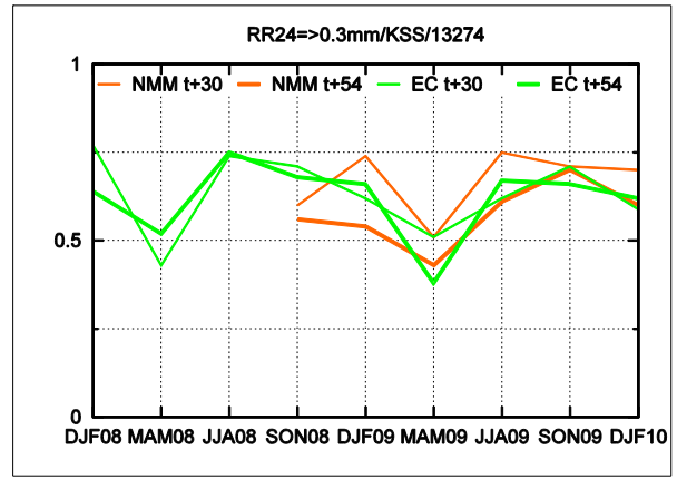
Fig.11-12 FBI and KSS of ECMWF 24h precipitation forecast (t+30h and t+54h) for seasons DJF08 to DJF10. Threshold is 0.3mm/24h. Comparison to WRF-NMM forecast from SON08 (Beograd - Karadordev park).
