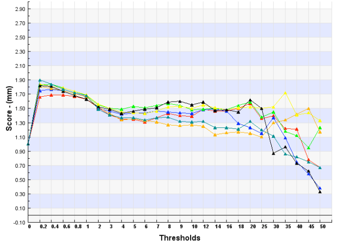
B=FBI ECMWF Seasonal Prec 24H Run 00 - Italy - 00 Run Stratification : All Italian Stations - Period: MAM 2009 n contingency table interval from 4340 to 4620
