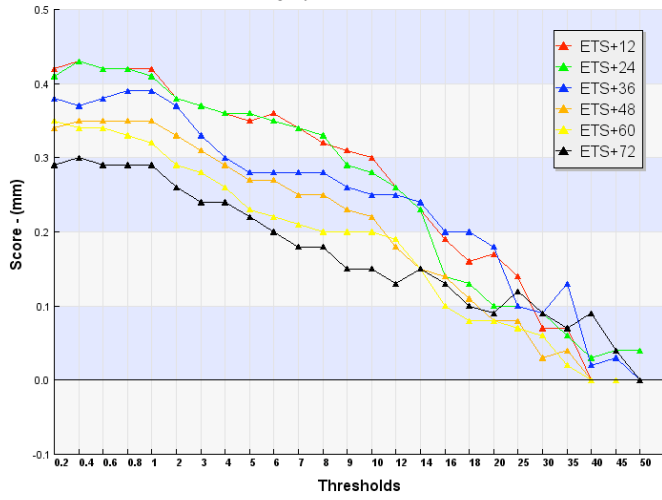
ETS COSMOME Seasonal Prec 12H Run 00 - Italy - 00 Run Stratification : All Italian Stations - Period: DJF 2008-2009 n contingency table interval from 4787 to 4868
