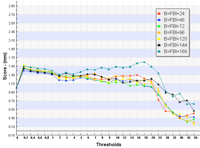
B=FBI ECMWF Seasonal Prec 24H Run 00 - Italy - 00 Run Stratification : All Italian Stations - Period: DJF 2008-2009 n contingency table interval from 2696 to 3033
