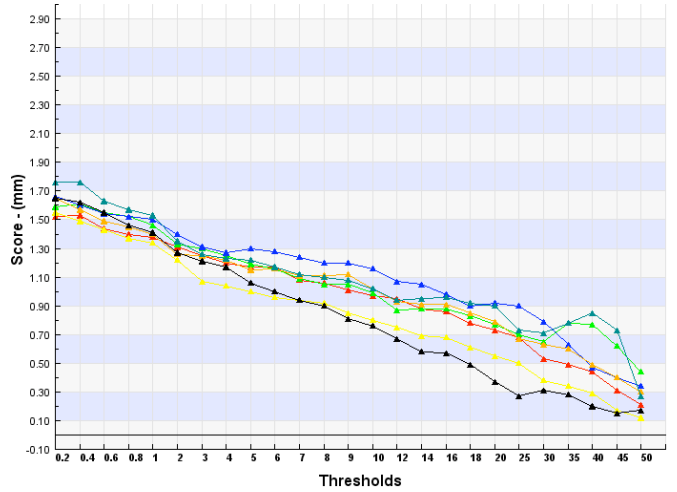
IFS Precipitation in 24 hours – FBI score
