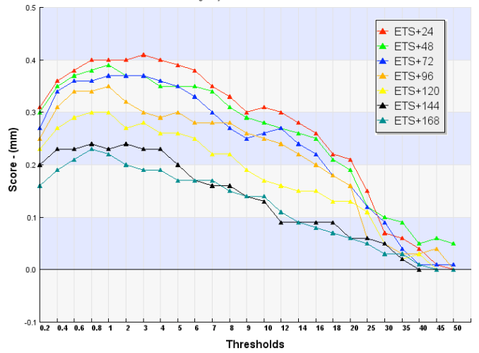
IFS Precipitation in 24 hours – ETS score
