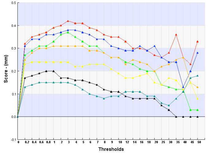
ETS ECMWF Seasonal Prec 24H Run 00 - Italy - 00 Run Stratification : All Italian Stations - Period: MAM 2009 n contingency table interval from 4340 to 4620
