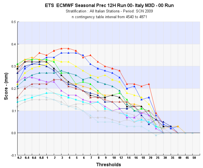
IFS Precipitation in 12 hours – ETS score
