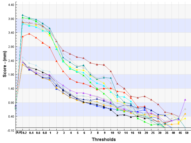
IFS Precipitation in 12 hours – FBI score
