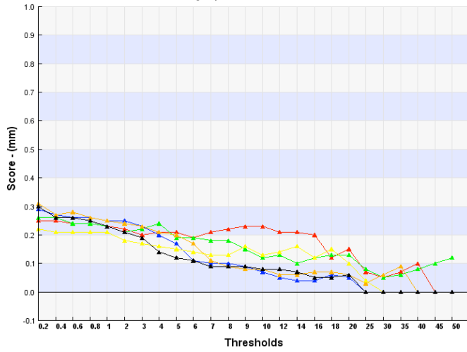
COSMO-ME Precipitation in 12 hours – ETS score
