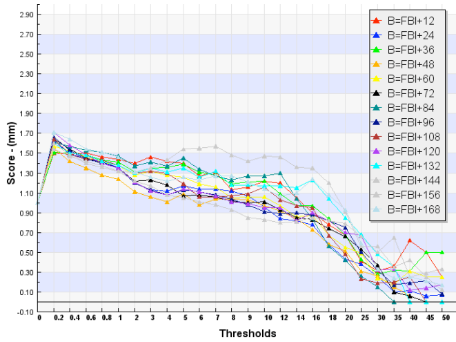
B=FBI ECMWF Seasonal Prec 12H Run 00- Italy - 00 Run
