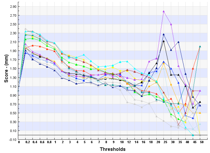
B=FBI ECMWF Seasonal Prec 12H Run 00- Italy M3D - 00 Run
