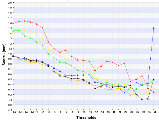
COSMO-ME Precipitation in 12 hours – FBI score
