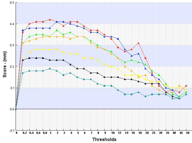
ETS ECMWF Seasonal Prec 24H Run 00 - Italy - 00 Run Stratification : All Italian Stations - Period: DJF 2008-2009 n contingency table interval from 2696 to 3033
