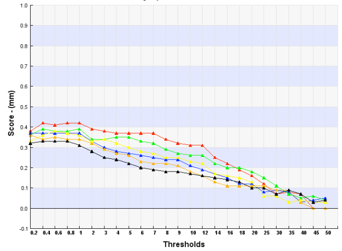
COSMO-ME Precipitation in 12 hours – ETS score
