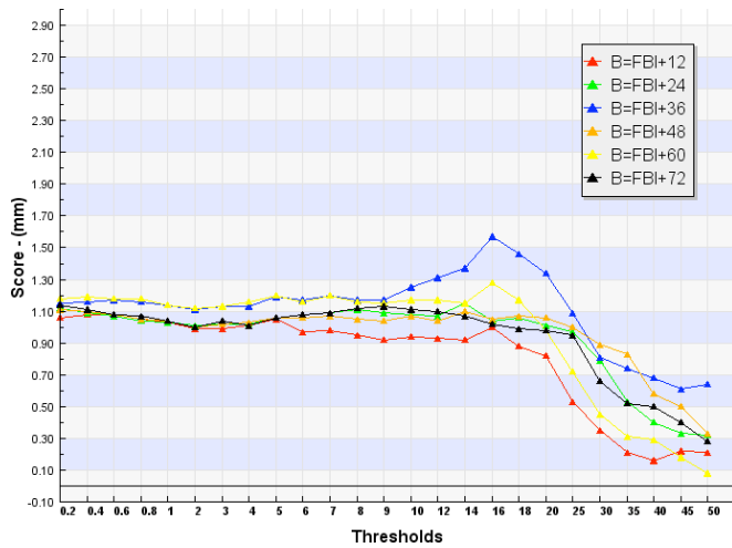
B=FBI COSMOME Seasonal Prec 12H Run 00 - Italy - 00 Run
