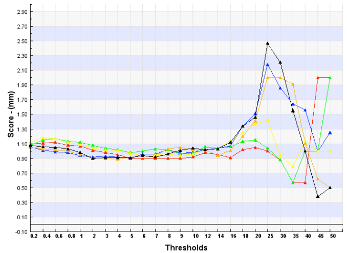
B=FBI COSMOME Seasonal Prec 12H Run 00 M3D-Italy - 00 Run
