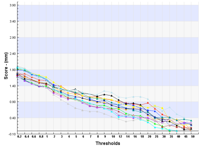
IFS Precipitation in 12 hours – FBI score
