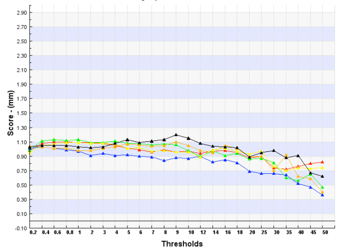
COSMO-ME Precipitation in 12 hours – FBI score
