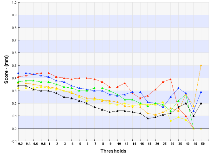
ETS COSMOME Seasonal Prec 12H Run 00 - Italy - 00 Run Stratification : All Italian Stations - Period: MAM 2009 n contingency table interval from 5029 to 5086
