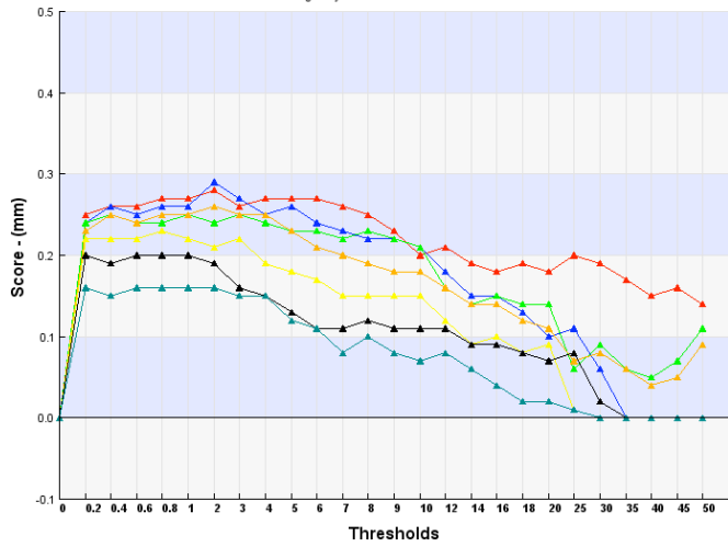
IFS Precipitation in 24 hours – ETS score
