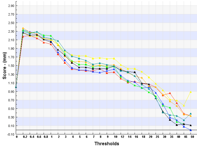
IFS Precipitation in 24 hours – FBI score
