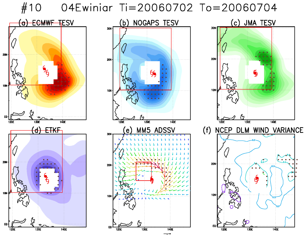
Figure 3: Same as Fig. 2, but for the small-domain common targeted location comparison and the brown dots represent X=31 grid points with highest value.
