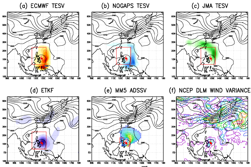
Figure 10: The sensitivities of (a) ECSV, (b) NGPSV, (c) JMASV, (d) ETKF, (e) ADSSV and (f) NCVAR superposed with the geopotential height field (contour interval of 60 gpm) from NCEP FNL at 500 hPa of case # 2, with 0000UTC 11 May as the observing time ( t_a ). Except for (f), the verifying areas of the other 5 methods are shown as the red squares in (a)-(e). The JTWC best track at t_a are denoted by the solid typhoon symbols.
