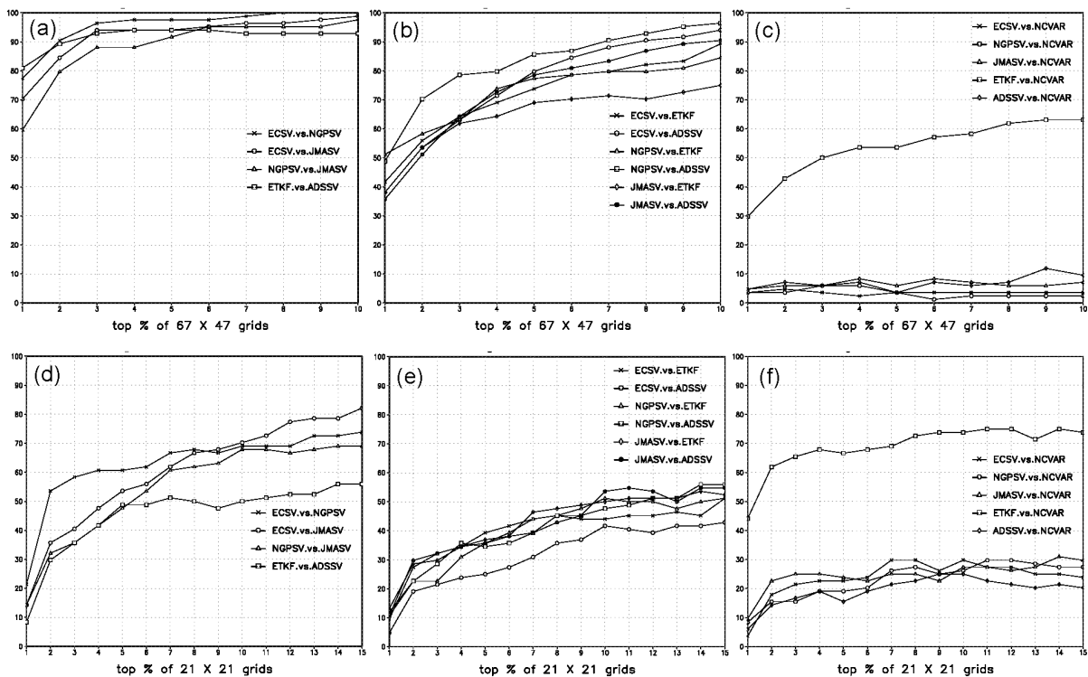
Figure 4: The ordinate shows the distribution of percentage among the 84 cases with METS > 0 . The abscissa indicates the threshold (in percentage from 1 to 10) grid numbers of the total 67 \times 47 grid points in the large domain [(a)- (c)], and from 1-15% of the total 21 \times 21 grid points in the small domain [(d)- (f)]. To show the lines distinctly, the 15 pairs are shown in three groups. The comparison results of three TESVs and ETKF versus ADSSV are shown in (a) and (d). (b) and (e) exhibit the results of ETKF and ADSSV versus the three TESVs, while (c) and (f) show NCVAR versus other five methods.
