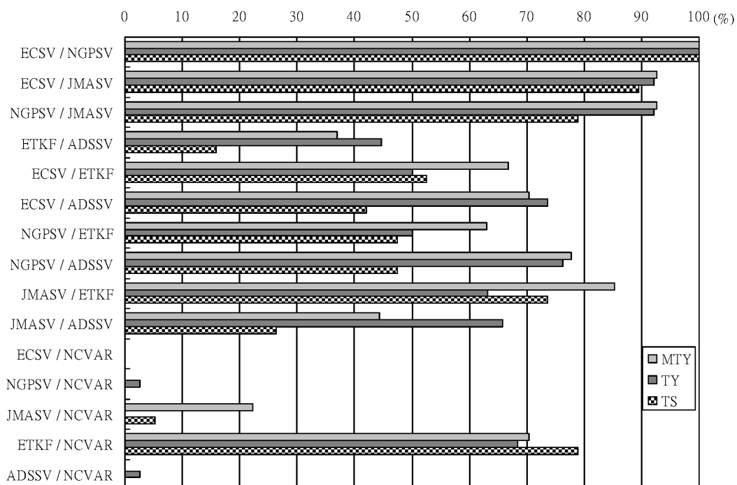
Figure 8: Percentage of cases with the Spearman rank correlation coefficient ( R_s ) set to be larger than 0.2. Results are shown for typhoons of three different intensity categories: 27 major typhoons (MTY), 38 typhoons (TY) and 19 tropical cyclones (TS).
