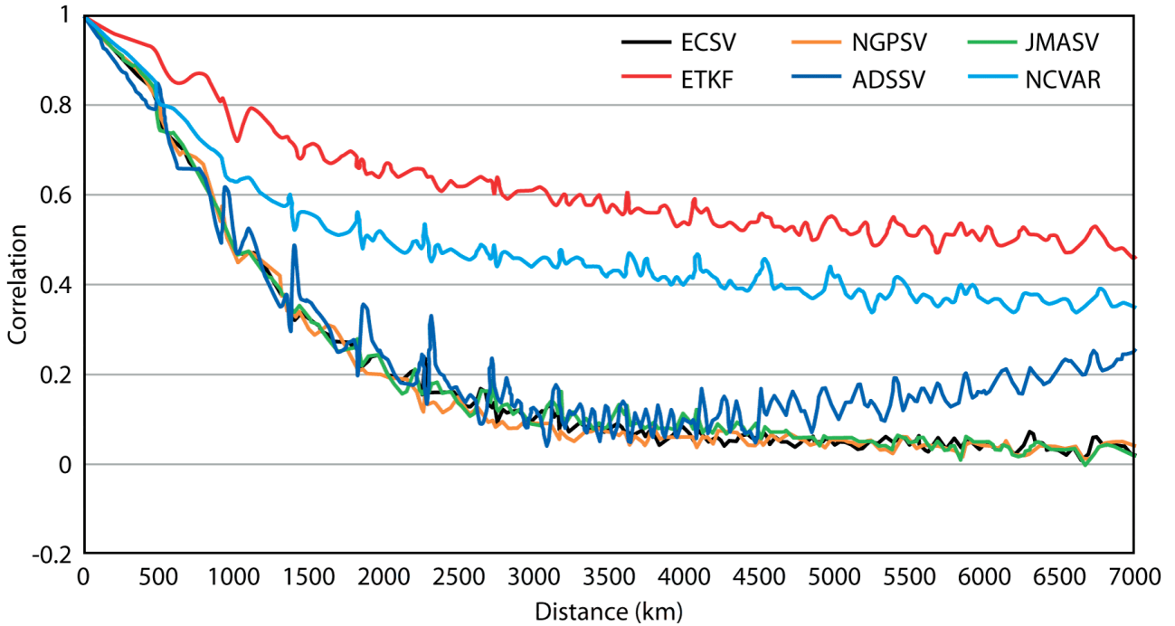
Figure B. 1: Correlation between points as the function of distance among all regions for the 6 targeted methods.
