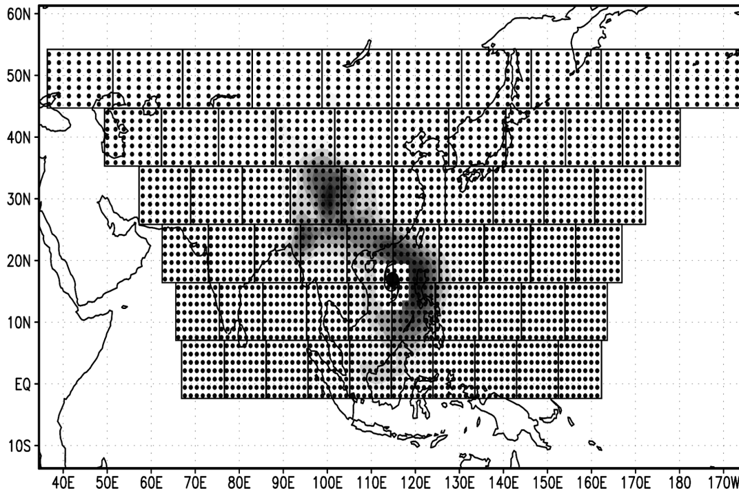
Figure 5: Regions to be ranked for NPGSV for case # 7 ( t_a = 0000 UTC 16 May 2006) in the large domain. Each of the Y = 60 square regions are plotted while each region consists of 7 \times 7 grid points at 150-km resolution.
