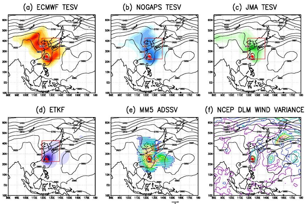
Figure 11: Same as Fig. 10, but for case #33 with 0000UTC 14 September as the observing time.
