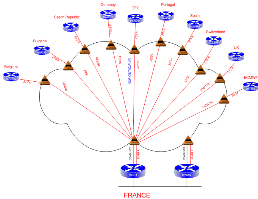
Figure 4-12: RMDCN Connections of France (source: www.ecmwf.int)
