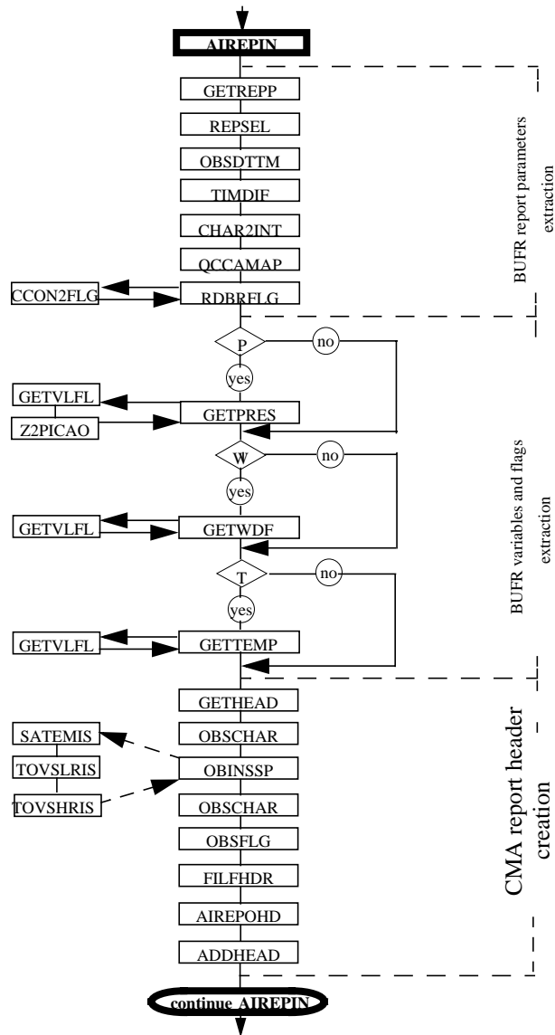
Figure 3.5 Subroutine AIREPIN flow diagram
